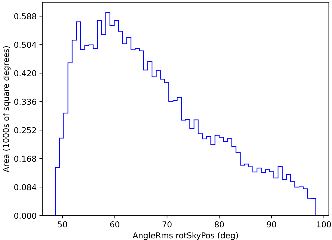
weather_cloudso8v3.4_10yrs WFD z band: AngleRms rotSkyPos
