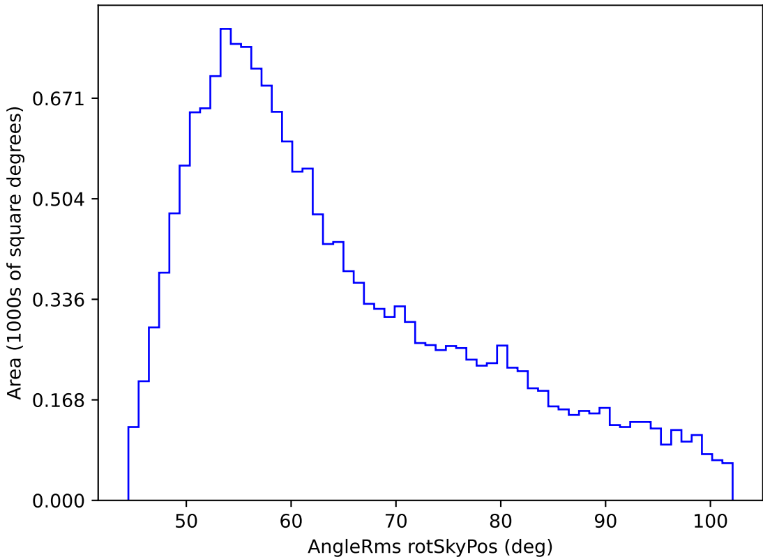
weather_cloudso8v3.4_10yrs WFD u band: AngleRms rotSkyPos
