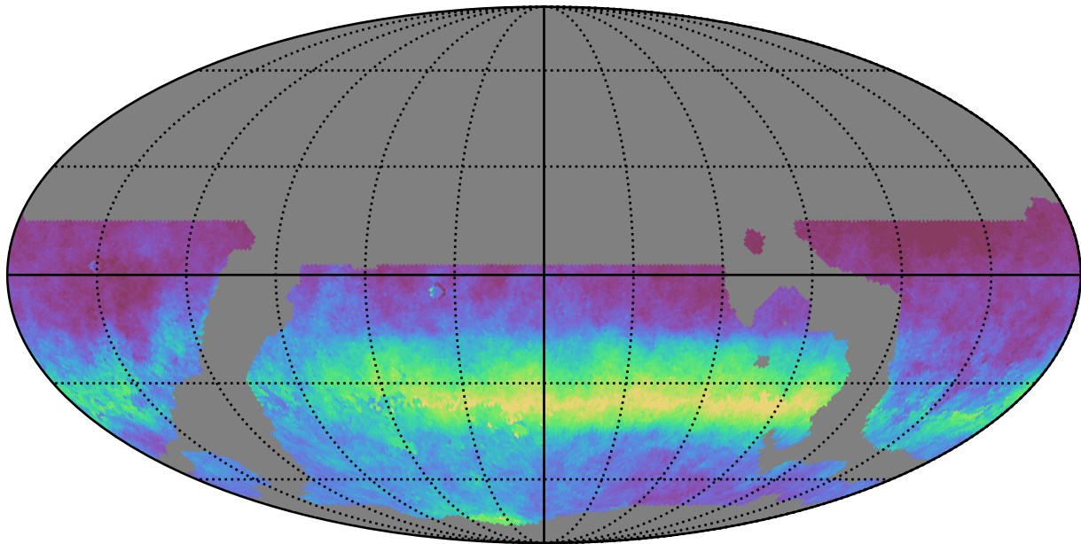
weather_cloudso8v3.4_10yrs WFD r band: AngleRms rotSkyPos
