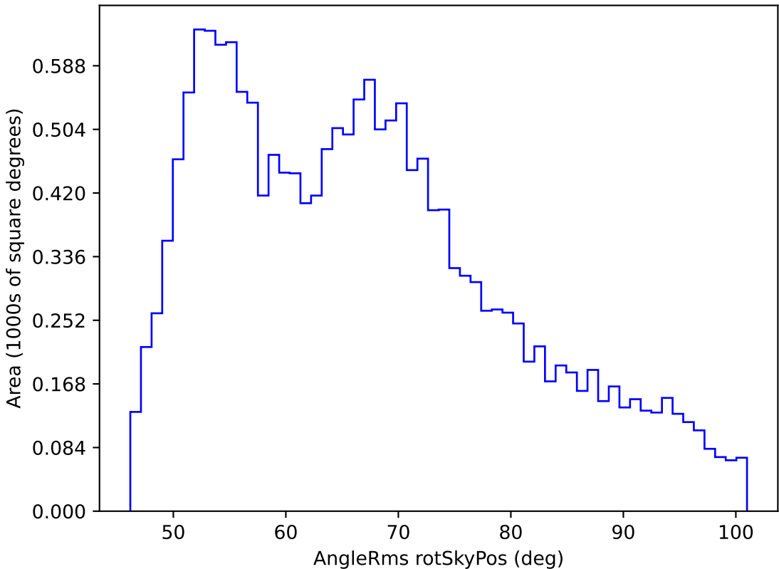
weather_cloudso8v3.4_10yrs WFD r band: AngleRms rotSkyPos
