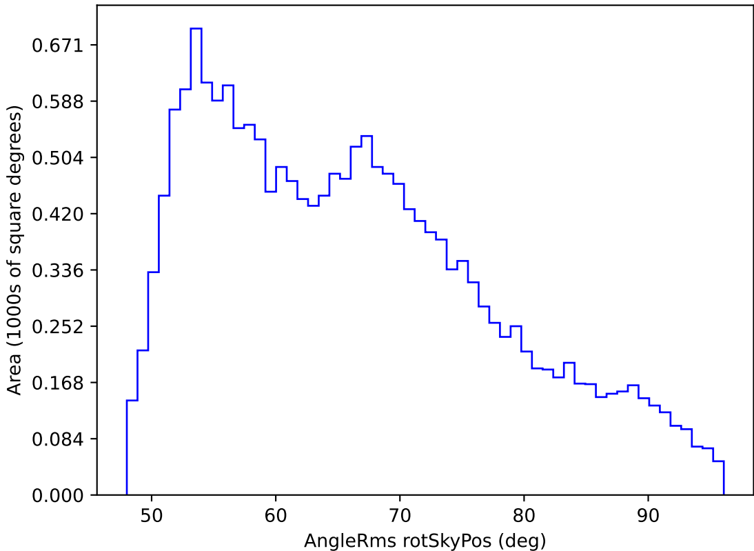
weather_cloudso8v3.4_10yrs WFD i band: AngleRms rotSkyPos
