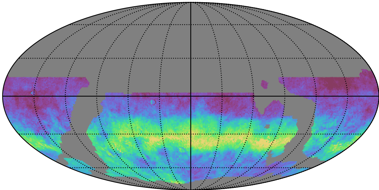
weather_cloudso8v3.4_10yrs WFD g band: AngleRms rotSkyPos
