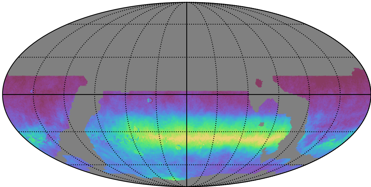
weather_cloudso8v3.4_10yrs WFD all bands: AngleRms rotSkyPos
