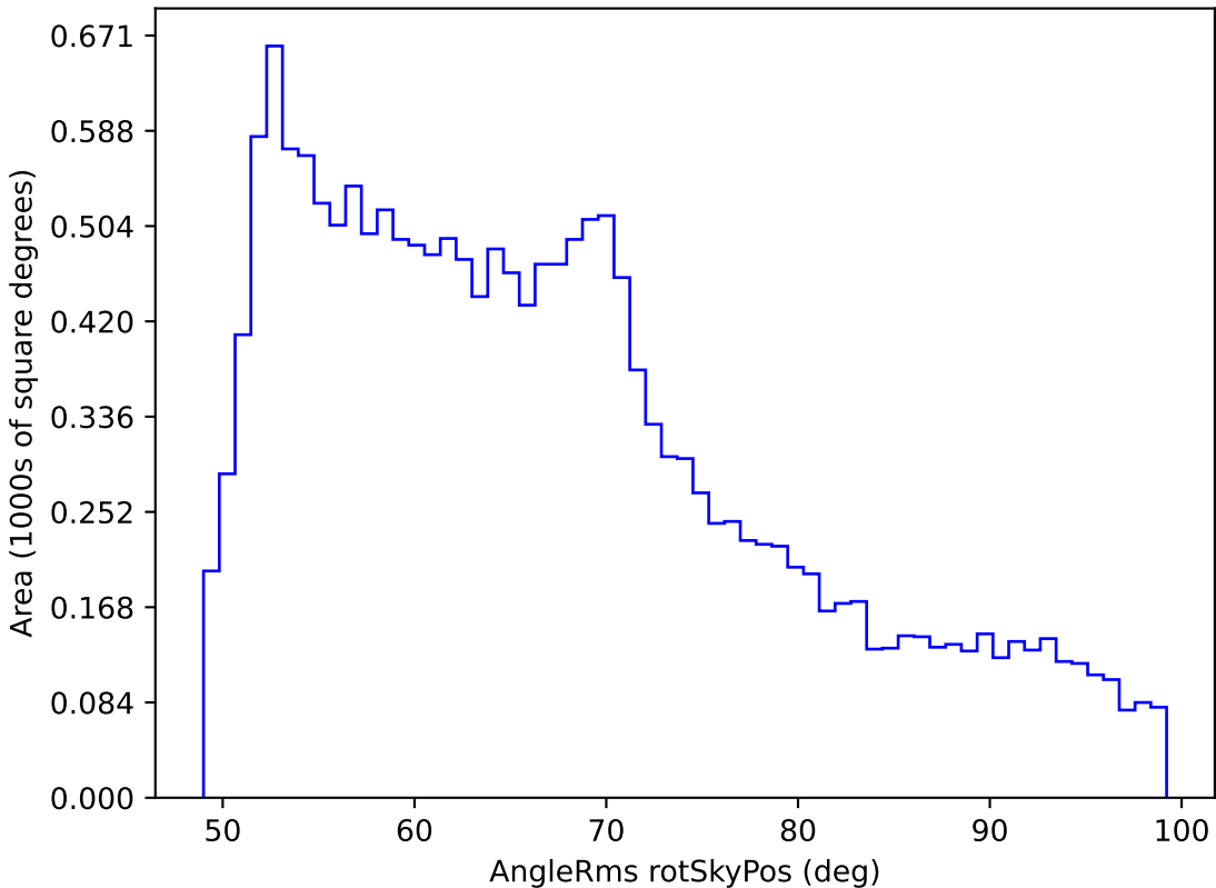
weather_cloudso8v3.4_10yrs WFD all bands: AngleRms rotSkyPos
