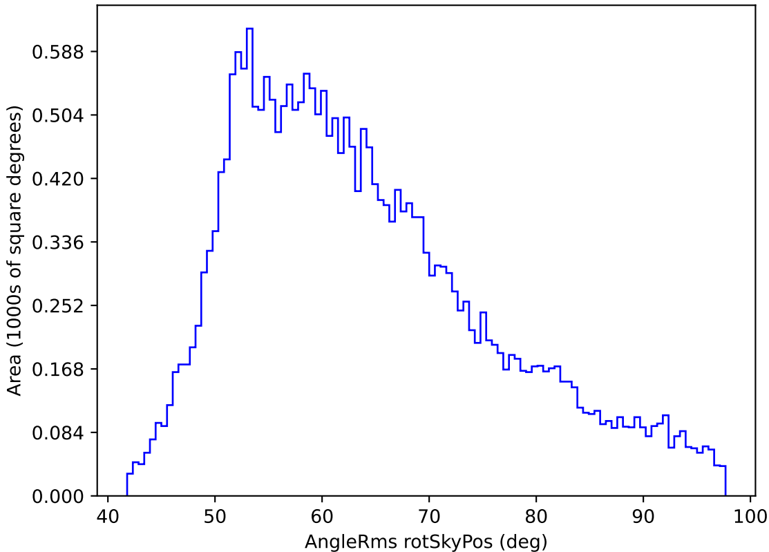
weather_cloudso8v3.4_10yrs All sky z band: AngleRms rotSkyPos
