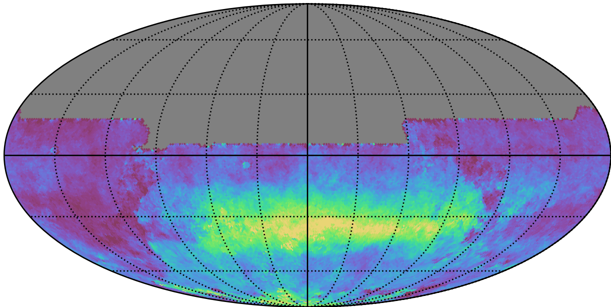
weather_cloudso8v3.4_10yrs All sky y band: AngleRms rotSkyPos
