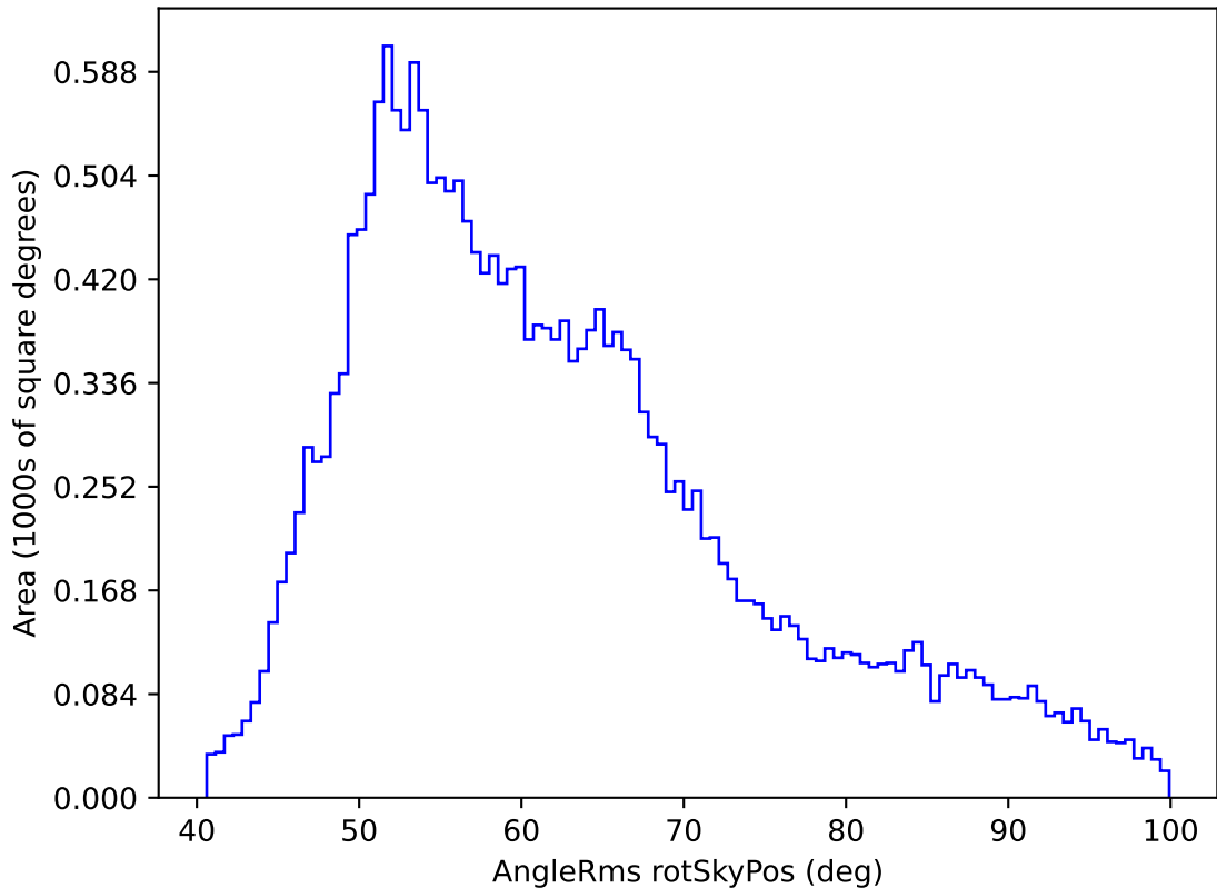
weather_cloudso8v3.4_10yrs All sky y band: AngleRms rotSkyPos
