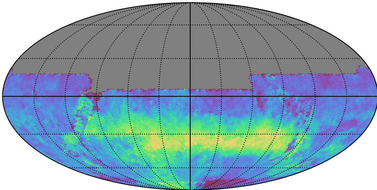
weather_cloudso8v3.4_10yrs All sky u band: AngleRms rotSkyPos
