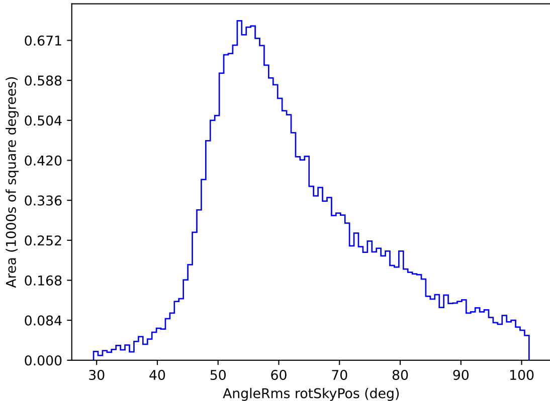
weather_cloudso8v3.4_10yrs All sky u band: AngleRms rotSkyPos
