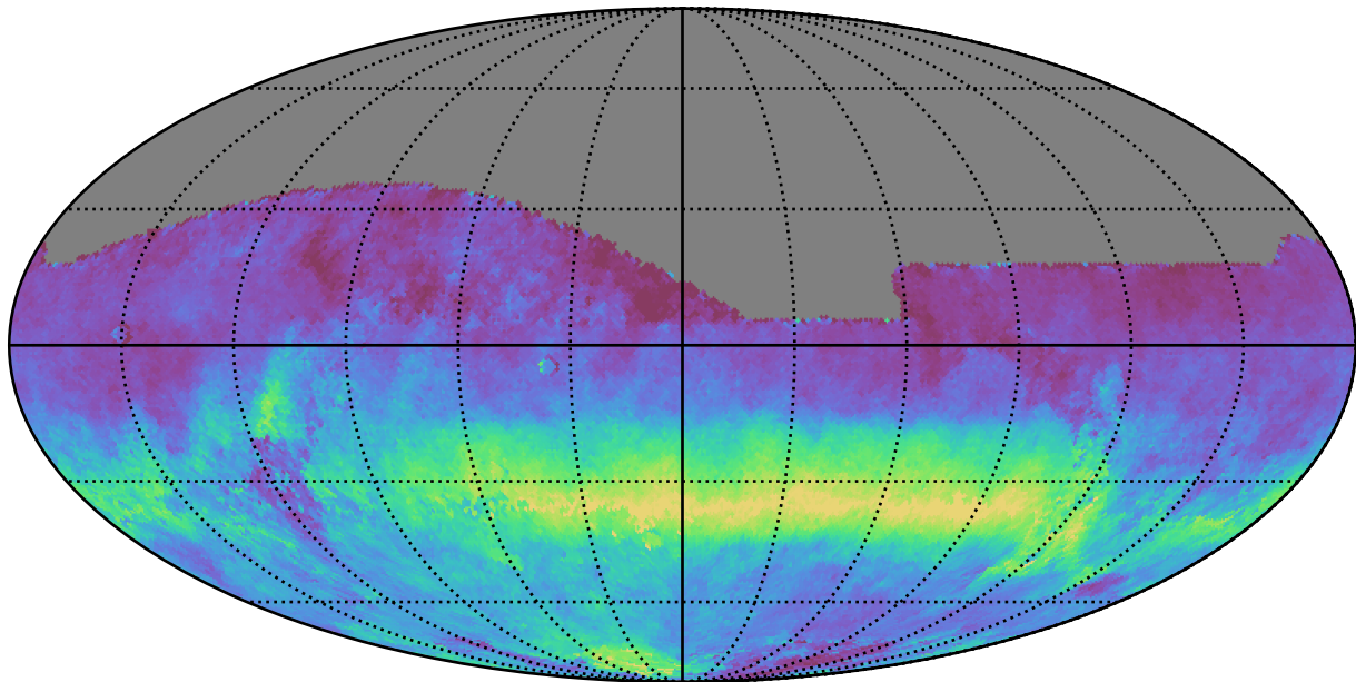
weather_cloudso8v3.4_10yrs All sky r band: AngleRms rotSkyPos
