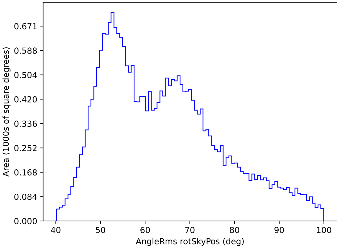
weather_cloudso8v3.4_10yrs All sky r band: AngleRms rotSkyPos
