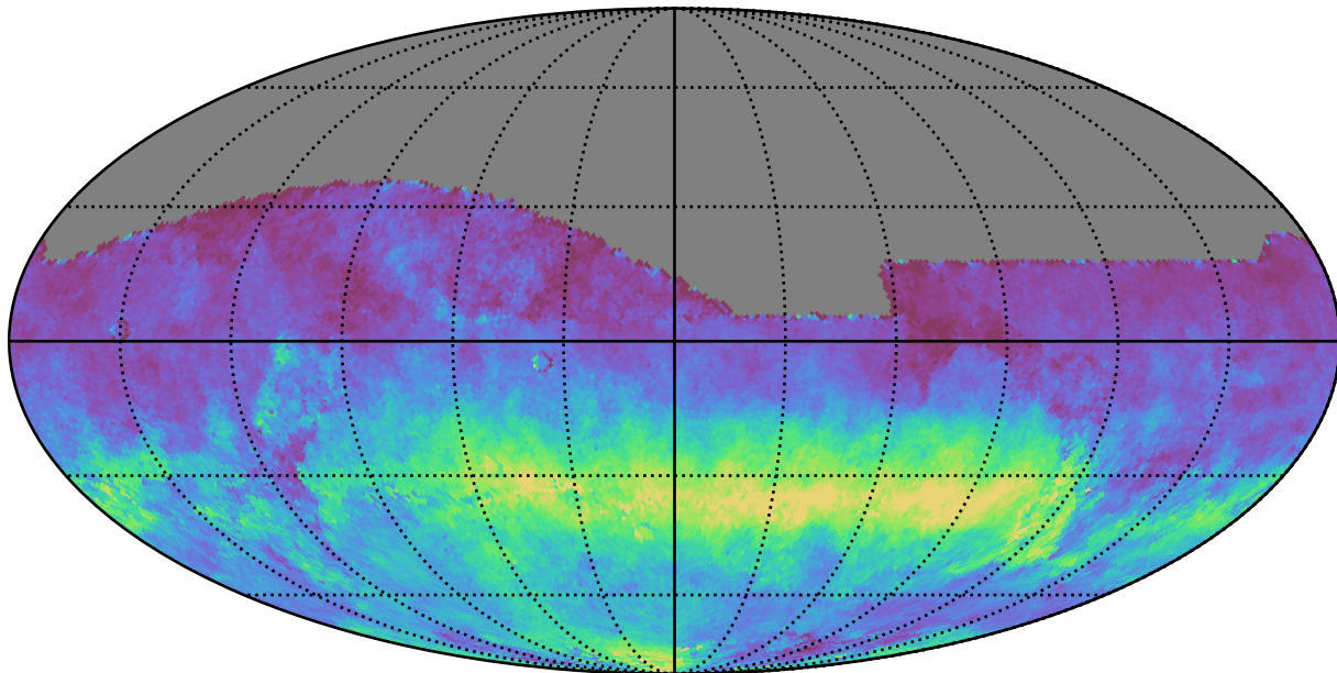
weather_cloudso8v3.4_10yrs All sky i band: AngleRms rotSkyPos
