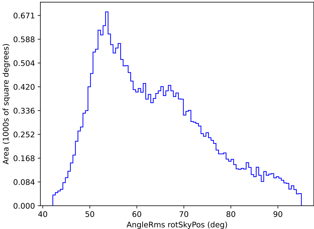
weather_cloudso8v3.4_10yrs All sky i band: AngleRms rotSkyPos
