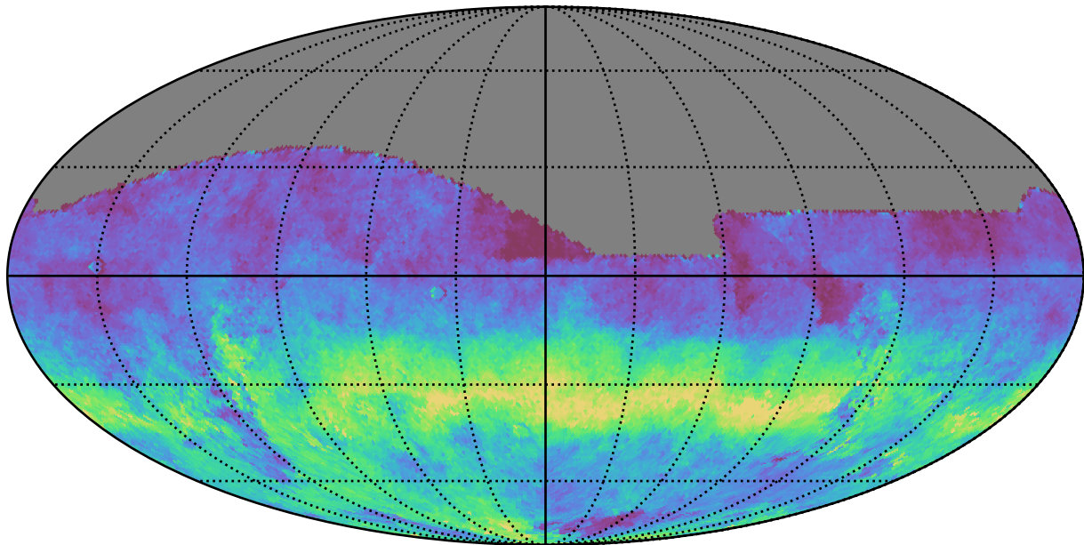
weather_cloudso8v3.4_10yrs All sky g band: AngleRms rotSkyPos
