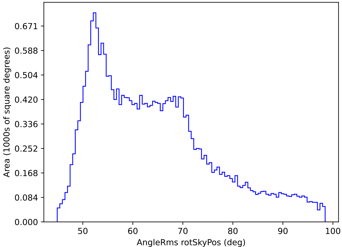
weather_cloudso8v3.4_10yrs All sky all bands: AngleRms rotSkyPos
