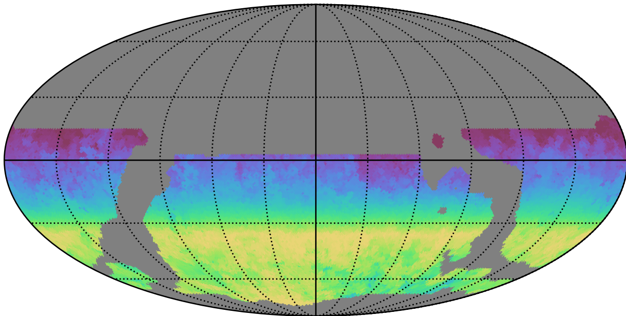
weather_cloudso8v3.4_10yrs WFD all bands: AngleRange rotSkyPos
