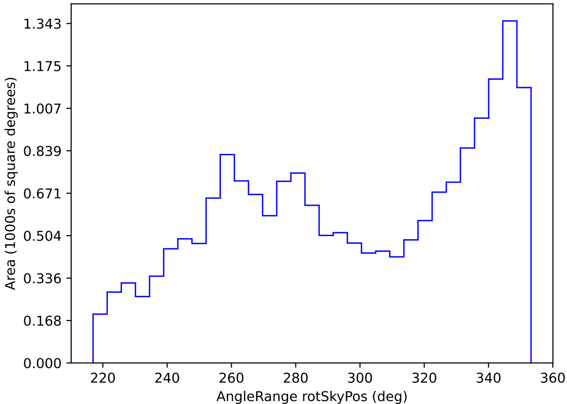
weather_cloudso8v3.4_10yrs WFD all bands: AngleRange rotSkyPos
