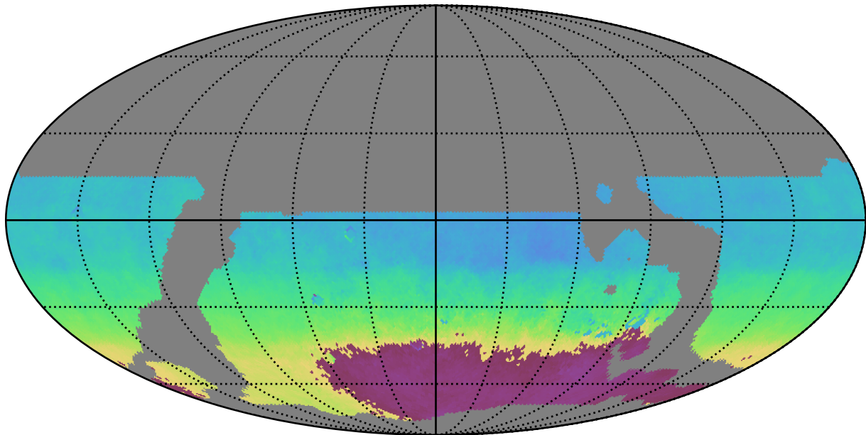
weather_cloudso8v3.4_10yrs WFD z band: AngleMean rotSkyPos
