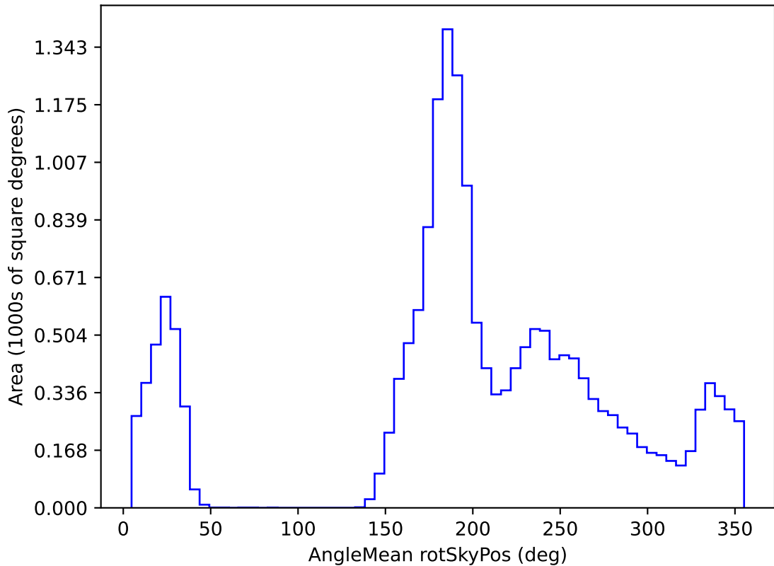
weather_cloudso8v3.4_10yrs WFD z band: AngleMean rotSkyPos
