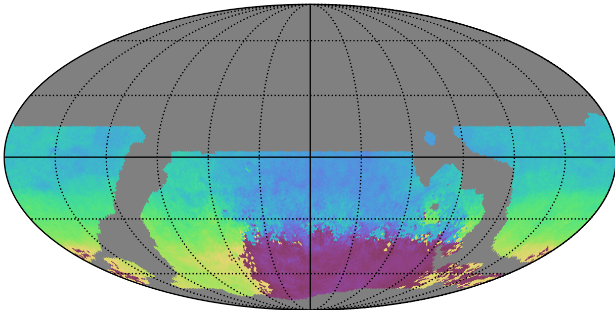
weather_cloudso8v3.4_10yrs WFD u band: AngleMean rotSkyPos
