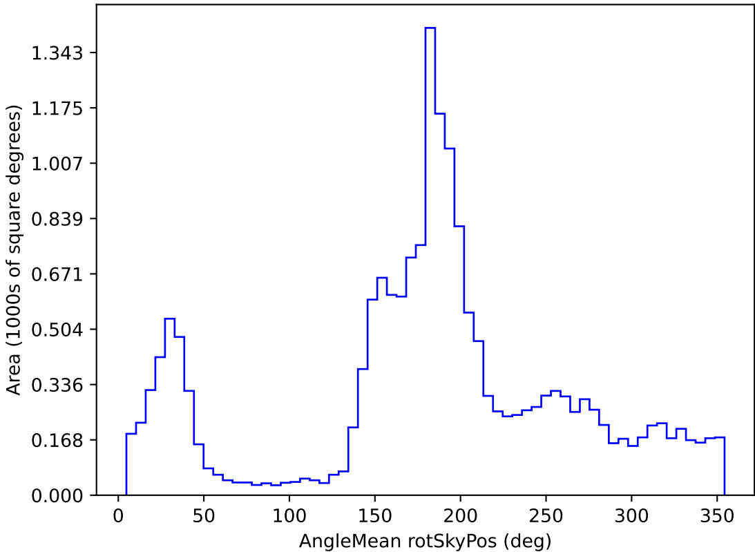
weather_cloudso8v3.4_10yrs WFD u band: AngleMean rotSkyPos
