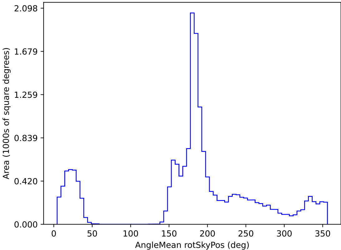
weather_cloudso8v3.4_10yrs WFD r band: AngleMean rotSkyPos
