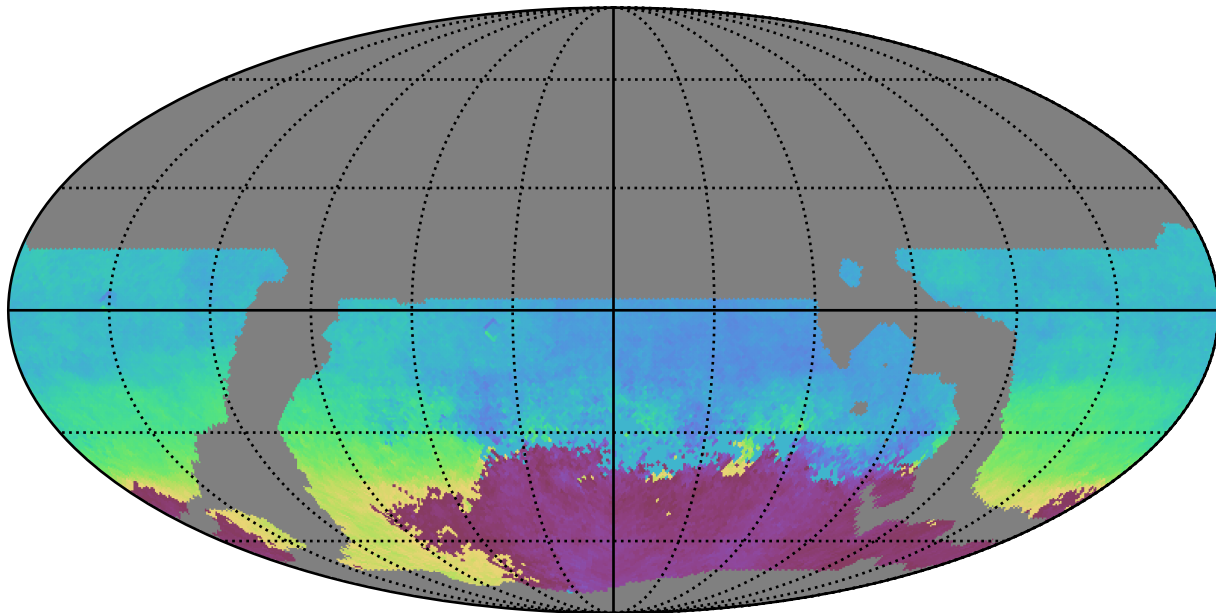
weather_cloudso8v3.4_10yrs WFD g band: AngleMean rotSkyPos
