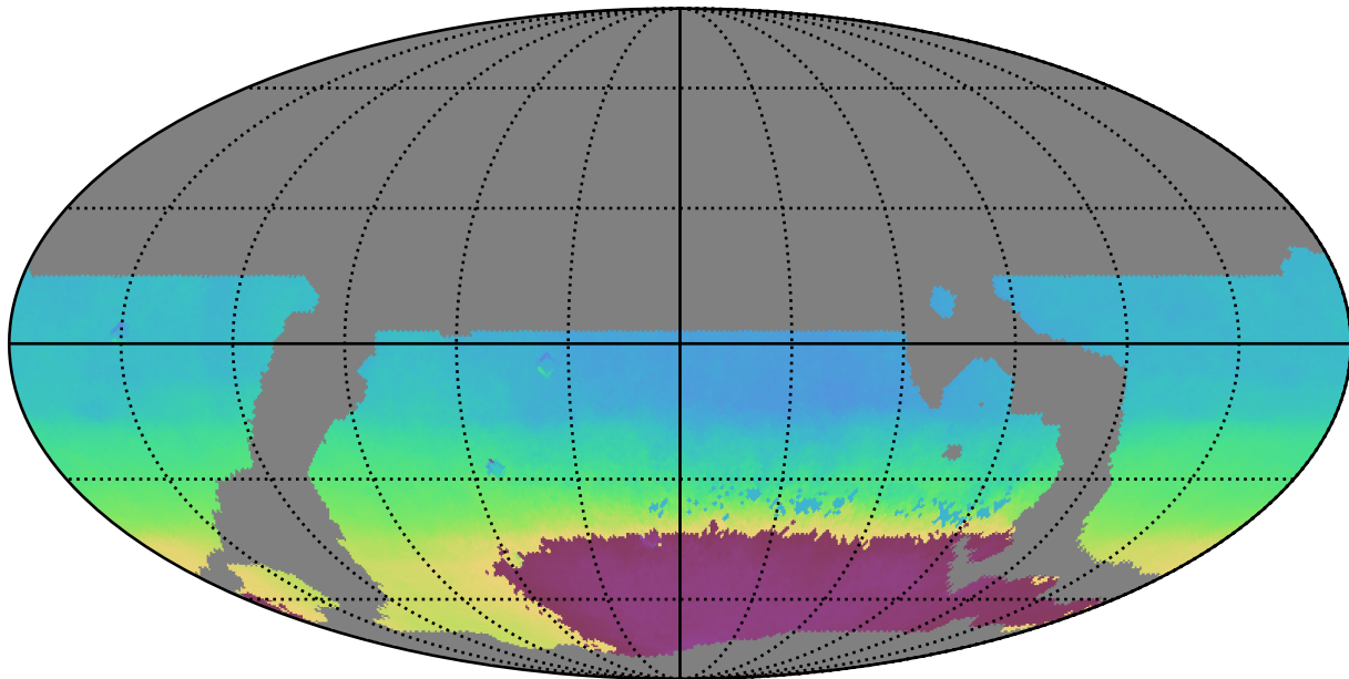
weather_cloudso8v3.4_10yrs WFD all bands: AngleMean rotSkyPos
