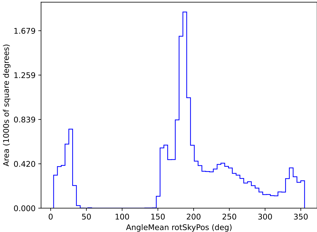
weather_cloudso8v3.4_10yrs WFD all bands: AngleMean rotSkyPos
