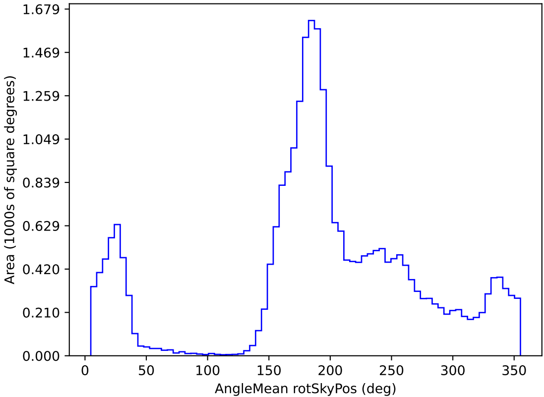
weather_cloudso8v3.4_10yrs All sky z band: AngleMean rotSkyPos
