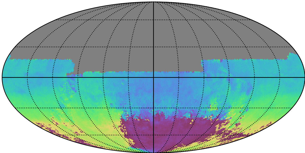
weather_cloudso8v3.4_10yrs All sky u band: AngleMean rotSkyPos
