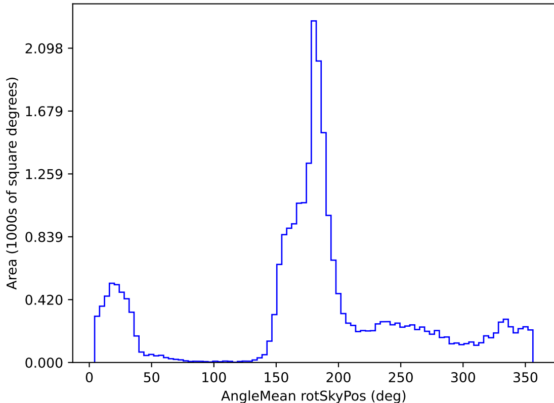
weather_cloudso8v3.4_10yrs All sky r band: AngleMean rotSkyPos
