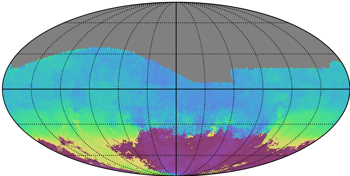
weather_cloudso8v3.4_10yrs All sky g band: AngleMean rotSkyPos
