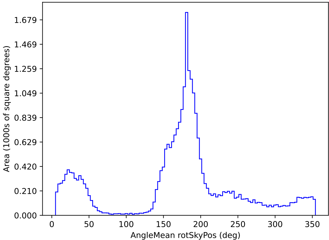
weather_cloudso8v3.4_10yrs All sky g band: AngleMean rotSkyPos
