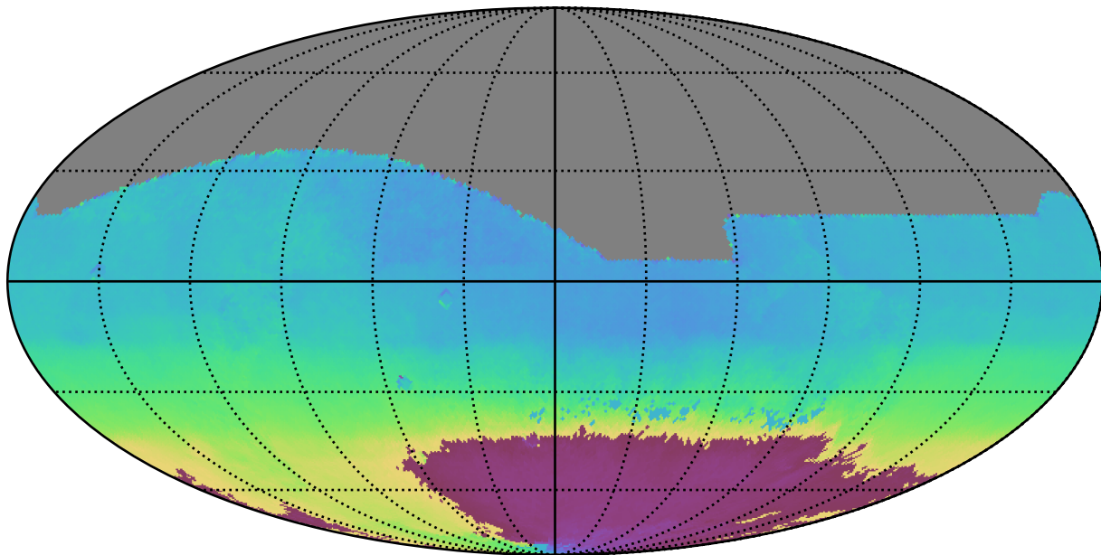
weather_cloudso8v3.4_10yrs All sky all bands: AngleMean rotSkyPos
