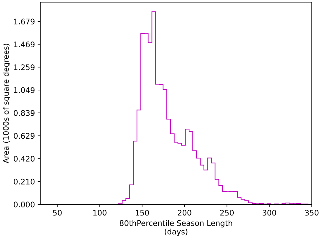
weather_cloudso8v3.4_10yrs WFD z band: 80thPercentile Season Length
