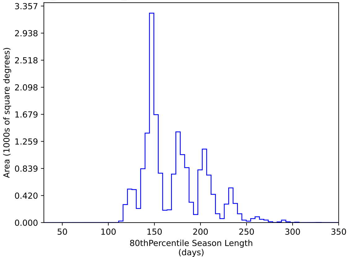
weather_cloudso8v3.4_10yrs WFD y band: 80thPercentile Season Length
