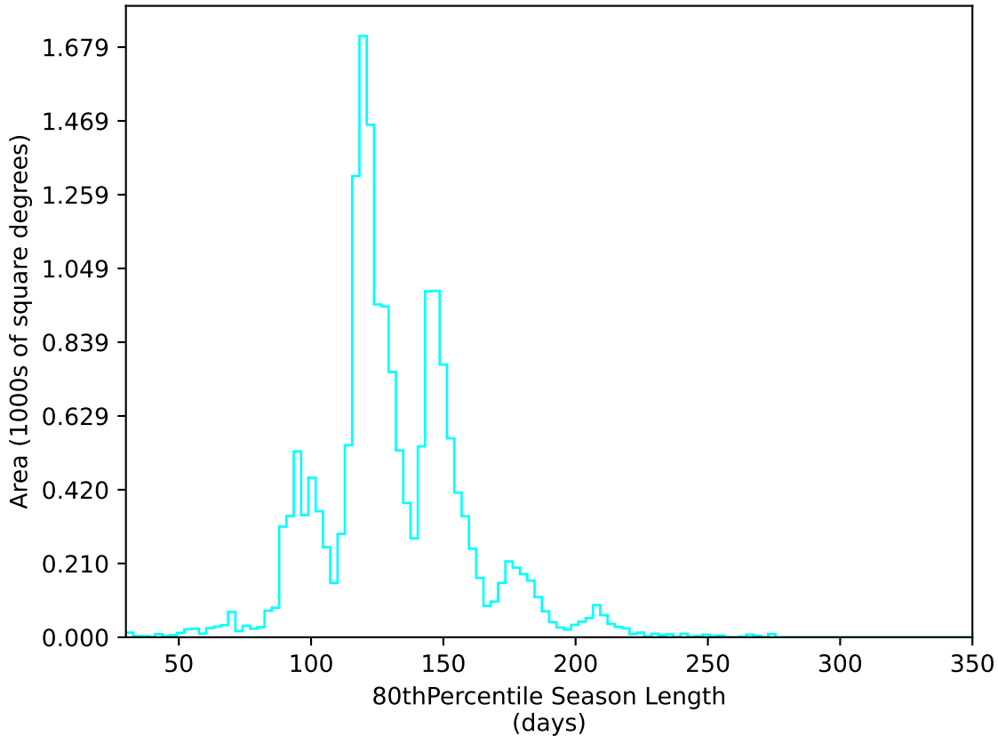
weather_cloudso8v3.4_10yrs WFD u band: 80thPercentile Season Length
