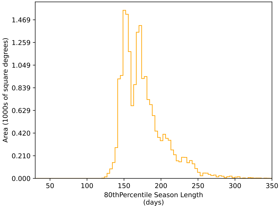
weather_cloudso8v3.4_10yrs WFD r band: 80thPercentile Season Length
