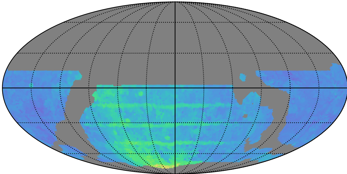
weather_cloudso8v3.4_10yrs WFD i band: 80thPercentile Season Length
