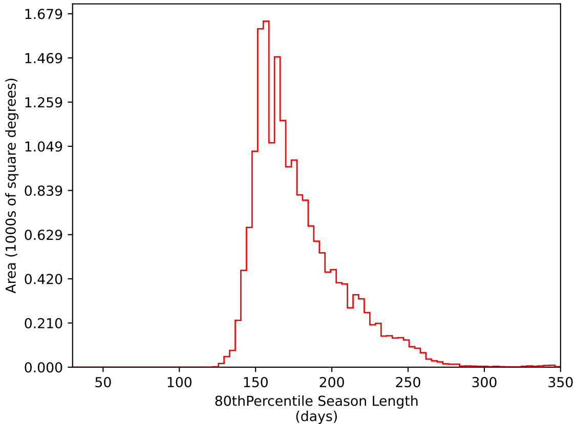
weather_cloudso8v3.4_10yrs WFD i band: 80thPercentile Season Length
