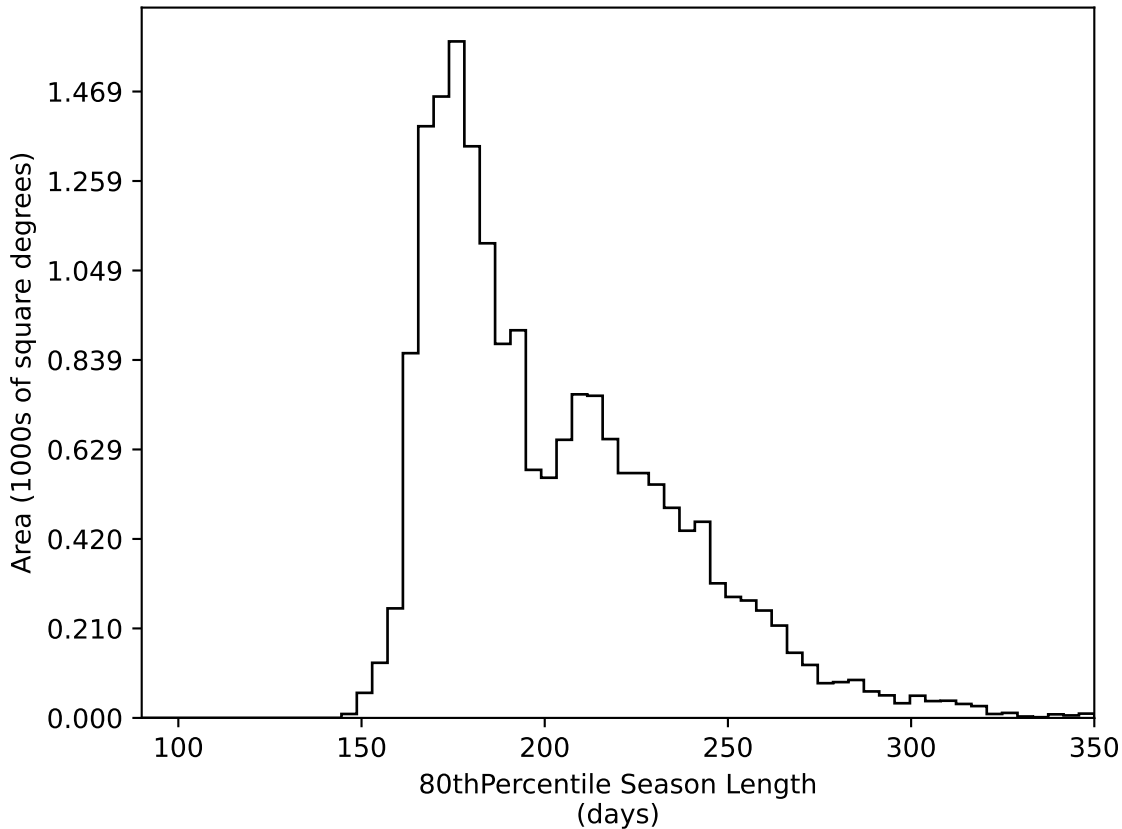
weather_cloudso8v3.4_10yrs WFD all bands: 80thPercentile Season Length
