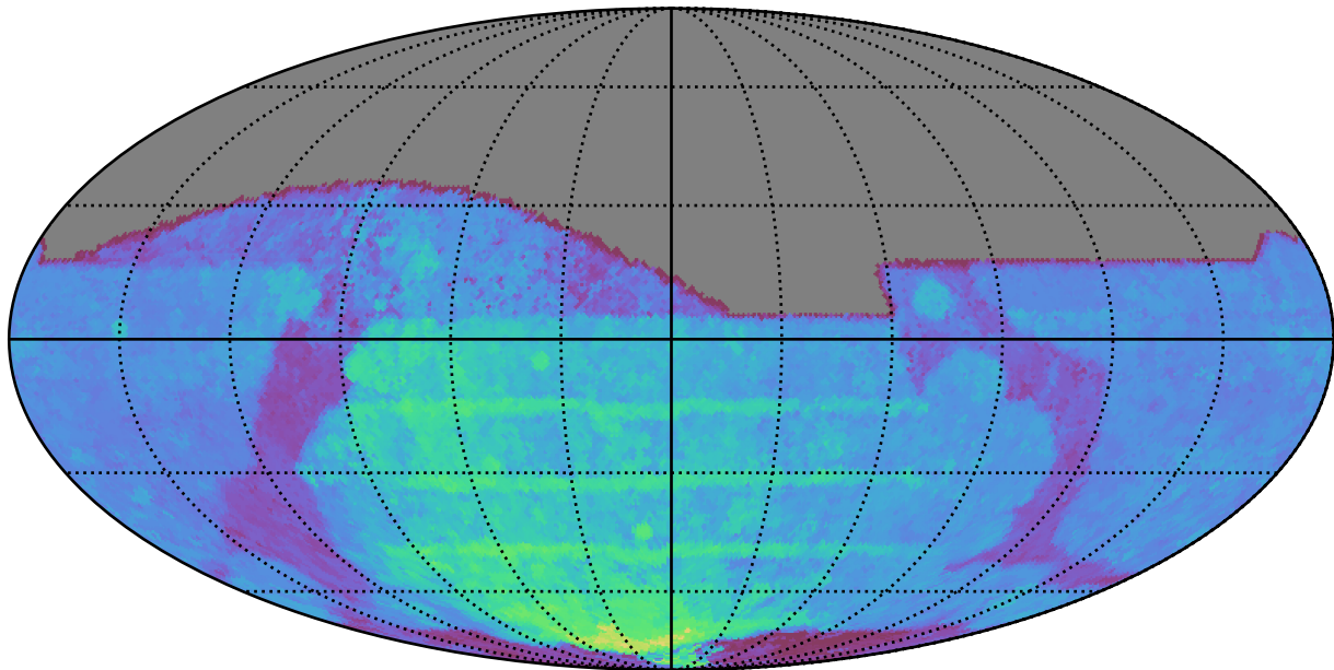
weather_cloudso8v3.4_10yrs All sky z band: 80thPercentile Season Length
