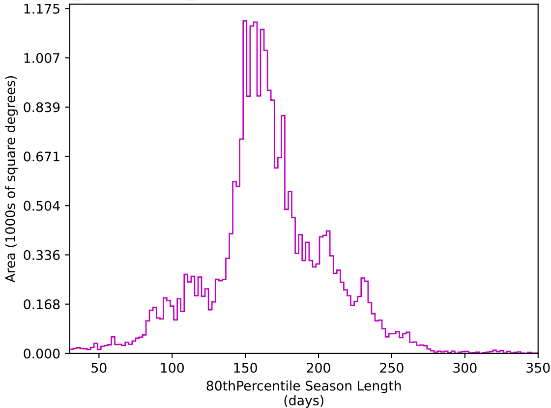
weather_cloudso8v3.4_10yrs All sky z band: 80thPercentile Season Length
