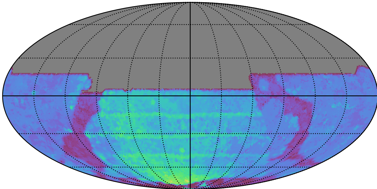
weather_cloudso8v3.4_10yrs All sky y band: 80thPercentile Season Length
