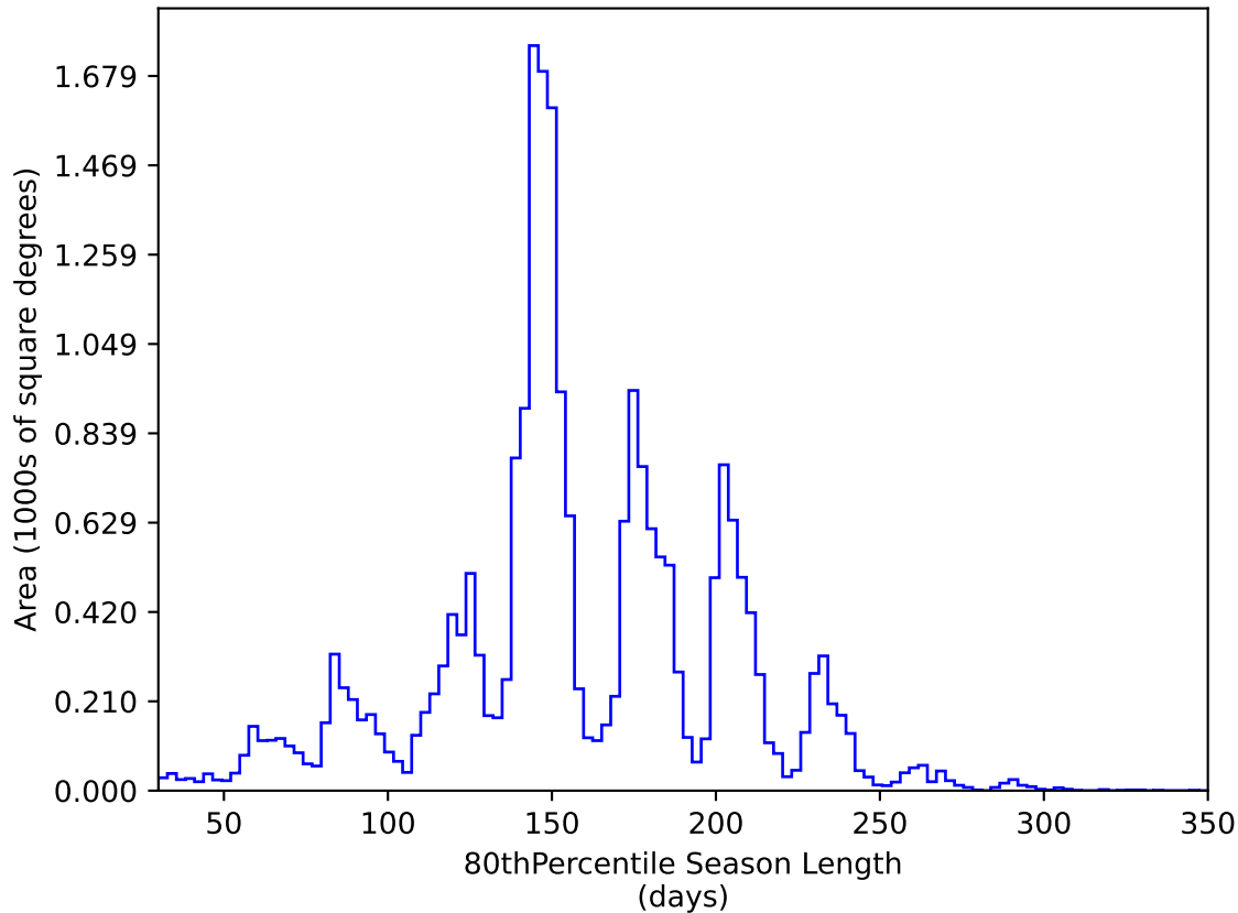
weather_cloudso8v3.4_10yrs All sky y band: 80thPercentile Season Length
