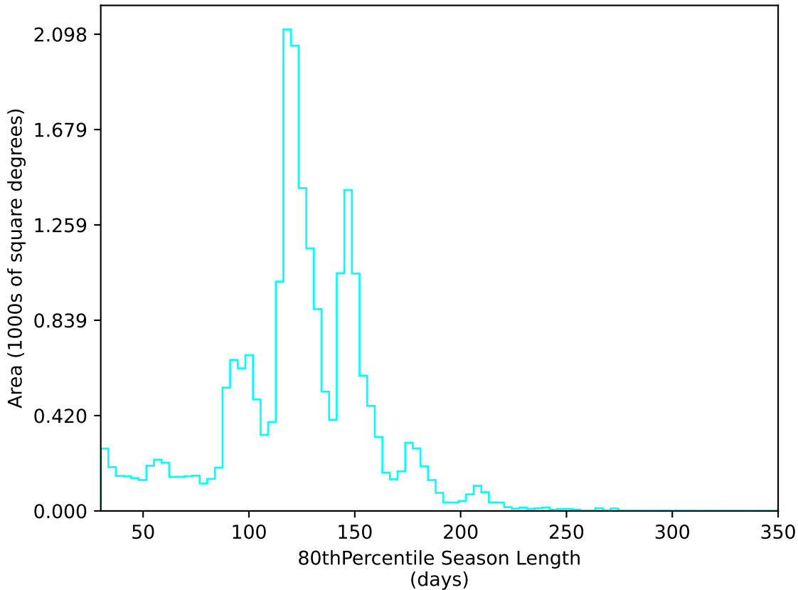
weather_cloudso8v3.4_10yrs All sky u band: 80thPercentile Season Length
