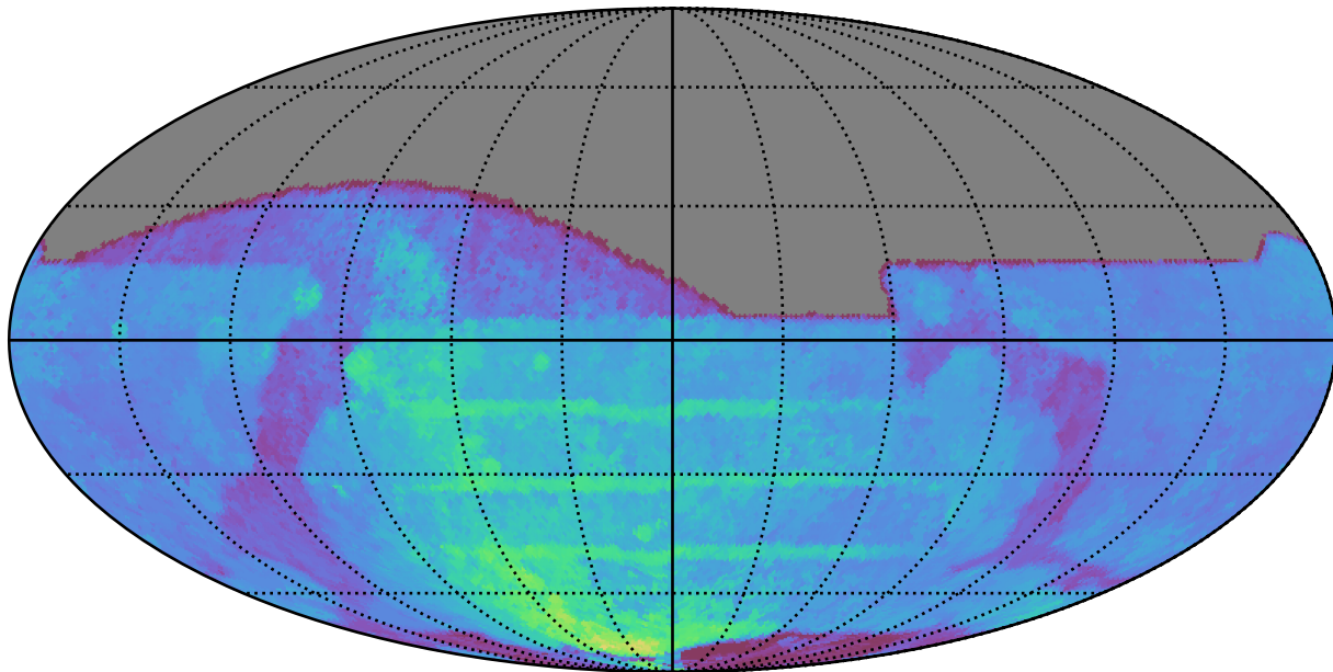
weather_cloudso8v3.4_10yrs All sky r band: 80thPercentile Season Length
