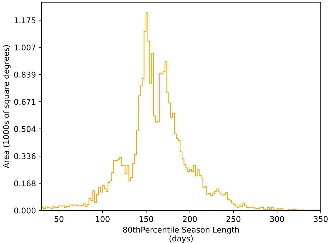
weather_cloudso8v3.4_10yrs All sky r band: 80thPercentile Season Length
