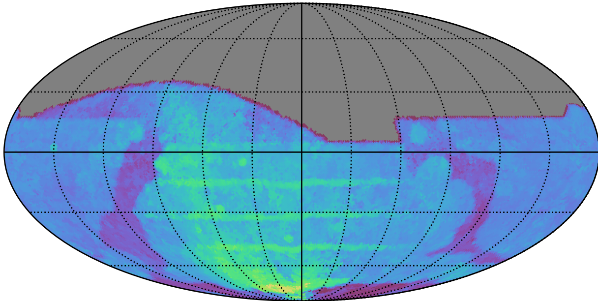
weather_cloudso8v3.4_10yrs All sky i band: 80thPercentile Season Length
